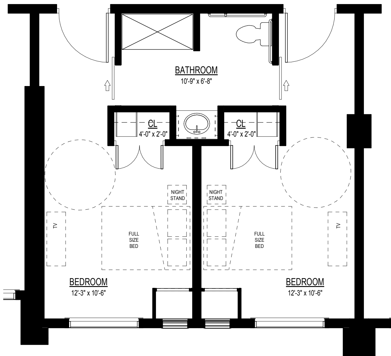
UNIT E - MC SEMI-PRIVATE 506 SF
